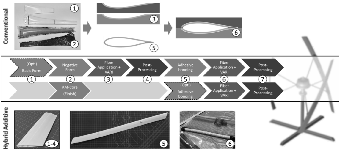
Fig. 5 Conventional vs. hybrid additive manufactured rotor blade
