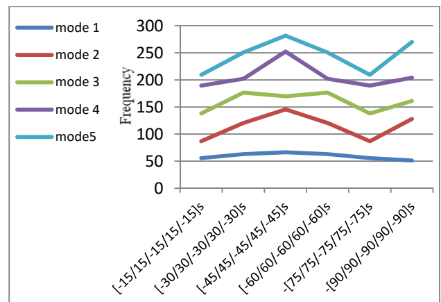
Fig. 8 Natural frequency (first five mode shape) of simply supported composite laminated plate with various layer orientations
