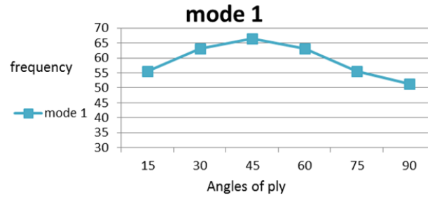
Fig. 7 Natural frequency (first mode shape) of simply supported composite laminated plate with various layer orientations
