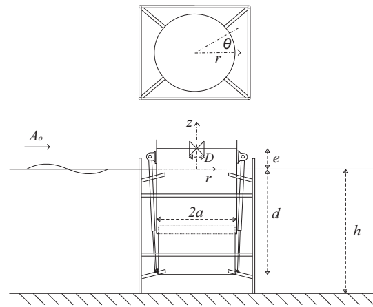
Fig. 1 Sketch of the OWC system [8]
