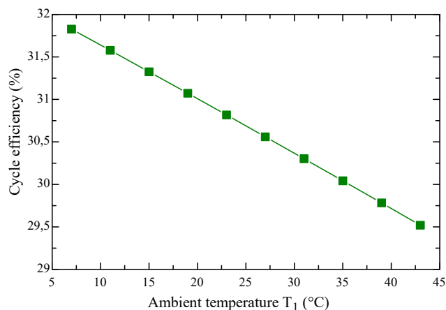
Fig. 3 Variation of cycle efficiency with ambient temperature
