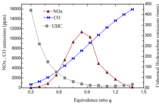
Fig. 8 The influence of equivalence ratio with NO x , CO, and UHC emissions
