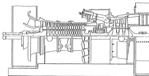
Fig. 1 GT design [5]
