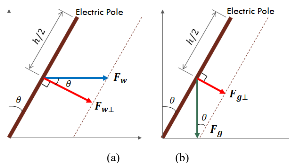
Fig. 1 (a) The wind force and (b) the gravitational force
