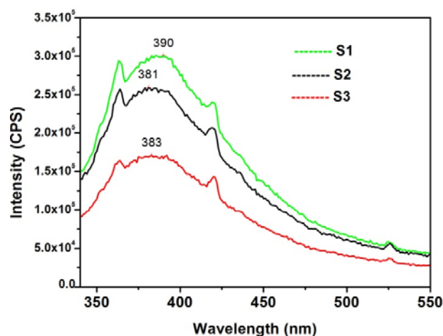
Fig. 4 PL spectra of ZnO/MPS nanocomposite irradiated with different doses of gamma radiation
