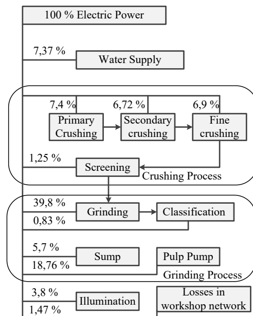
Fig. 1 A scheme of distribution of electric power consumption of the grinding process (when crushing proceeds the grinding process)
