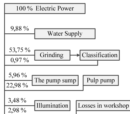
Fig. 2 A scheme of distribution of electric power consumption of the grinding process (when the crushing process is missing)
