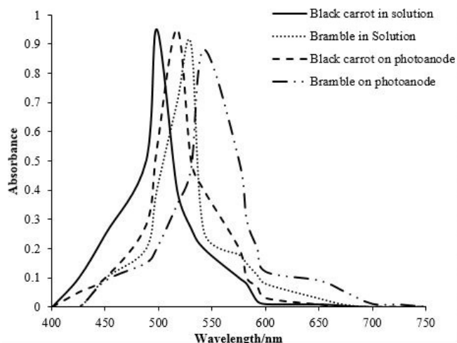
Fig. 2 UV-Vis absorption spectra for natural dyes
