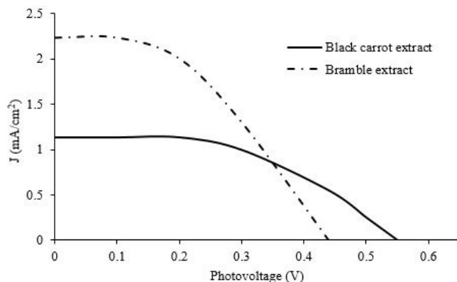
Fig. 3 Current density-voltage characteristics for black carrot and bramble
