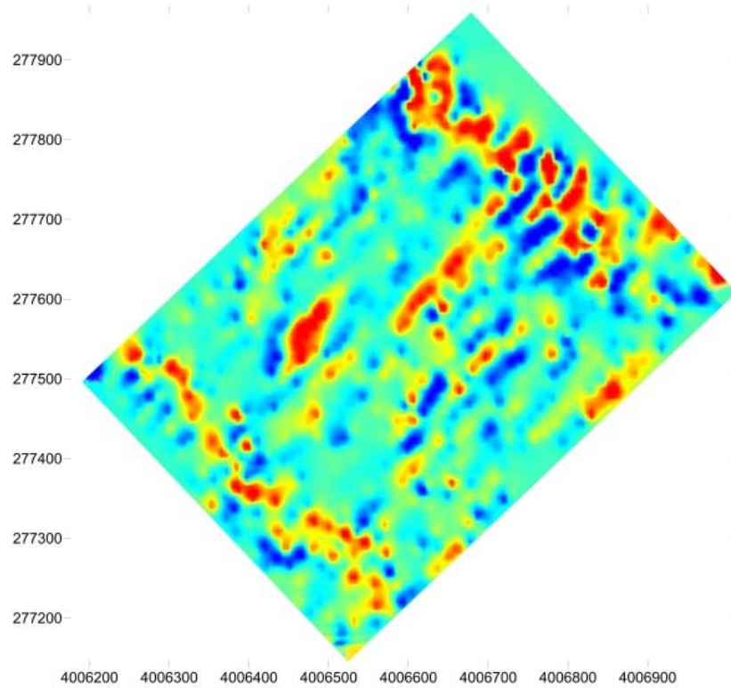
Fig. 4 Analytical signal map of study section
