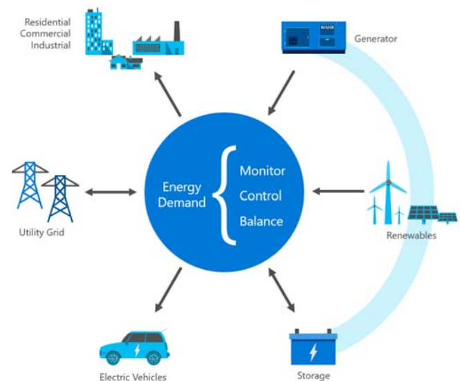
Fig. 1 Microgrid System
