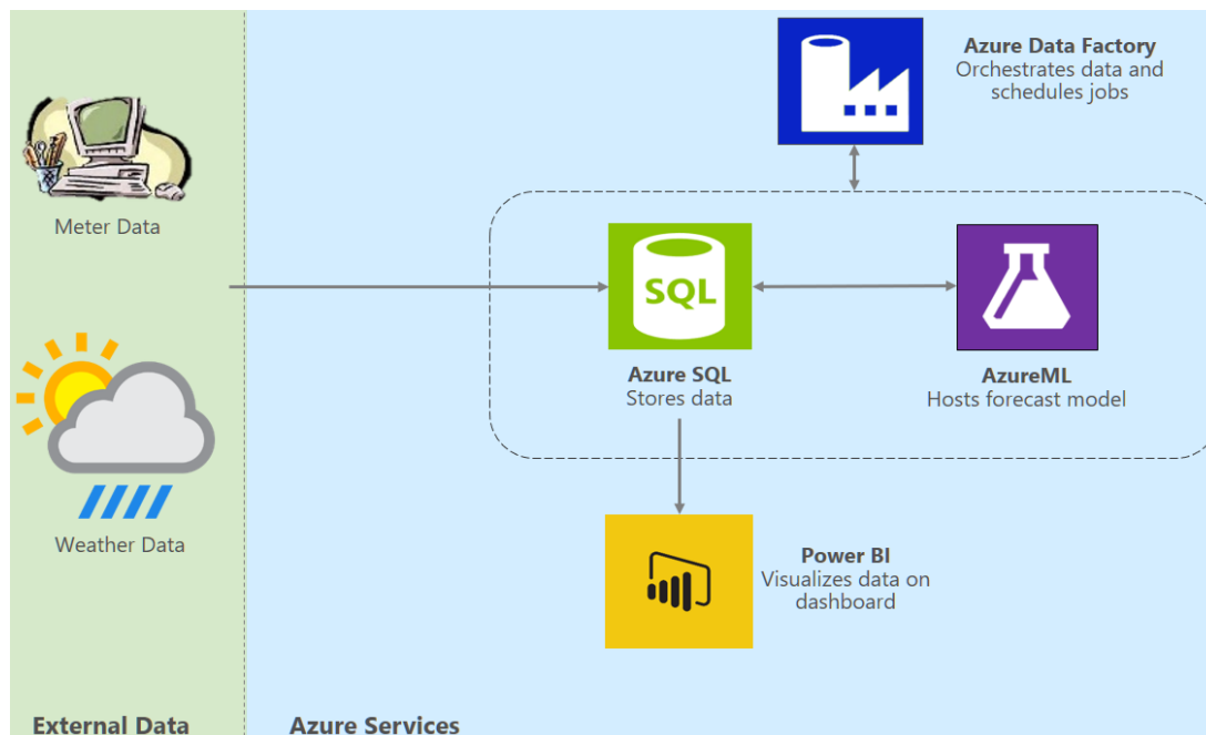
Fig. 8 Solution Architecture
