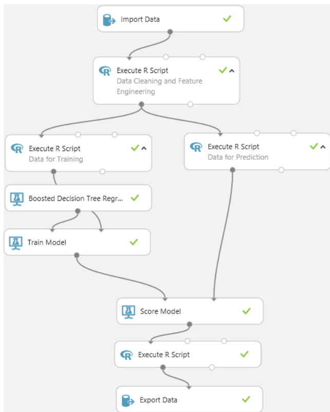
Fig. 6 Boosted Tree Regression Experiment for Steam Forecast
