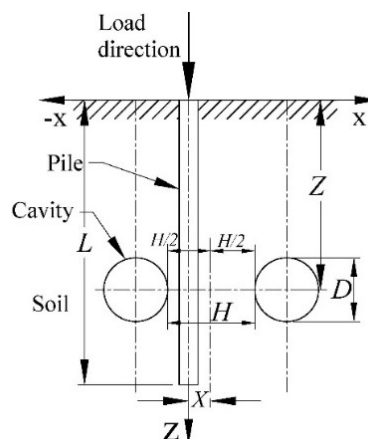
Fig. 3 Pile adjacent to twin cavities geometry
