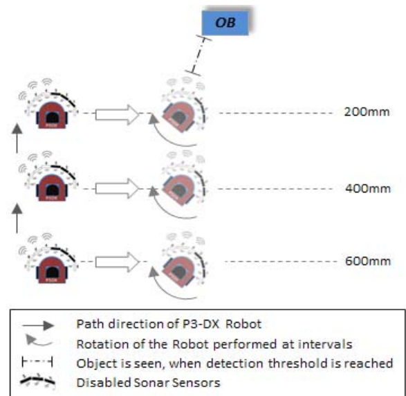
Fig. 10 When the robot has entered sonar failure mode; the robot is stopped and rotated at specific intervals during its task; an object OB can be discovered during a rotation event
