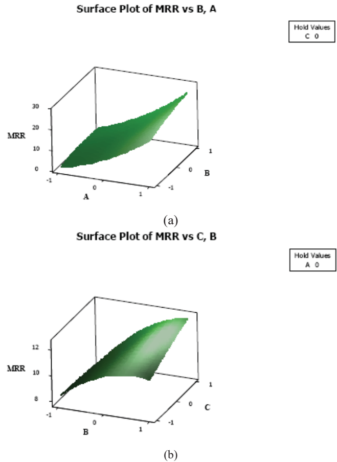
Fig. 1 Response surface plots of MRR for significant interactions (a). I \times T_{on} (b) T_{on} \times T_{off}
