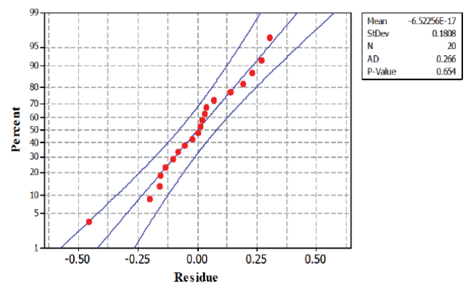
Fig. 2 AD plot for MRR
