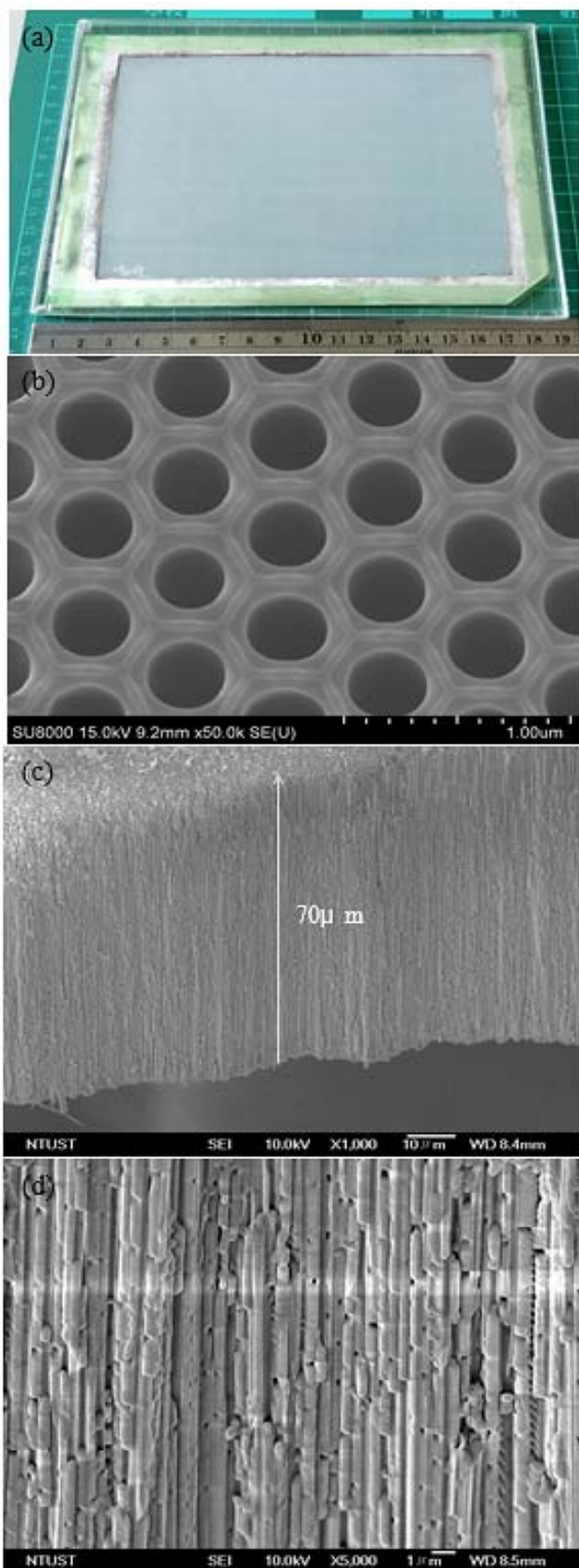
Fig. 5 AAO images; (a) large size of AAO film, (b) AAO micro-structure, (c) side view of CsI filling in the AAO film, (d) zoom in CsI filling in the AAO film
