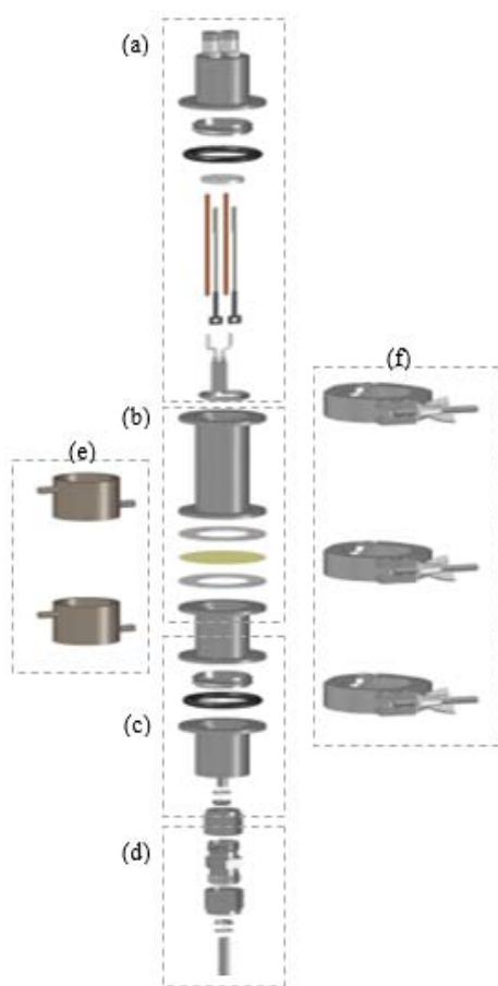
Fig. 3 The exploded diagram of vacuum inhalation chamber; (a) a vacuum heating chamber, (b) a sample placement cavity, (c) a vacuum chamber, (d) a vacuum connected group, (e) cooling rings, (f) clamps
