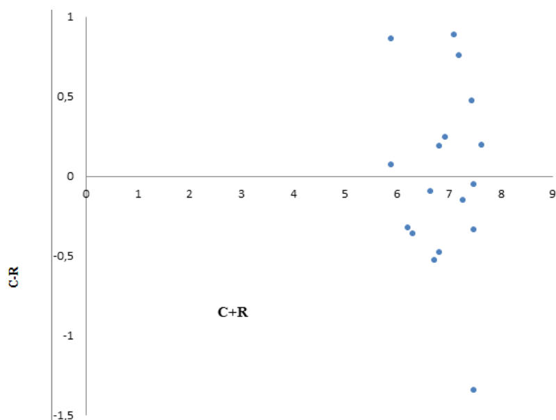
Fig. 1 Overall DEMATEL Prominence Casual Graph
