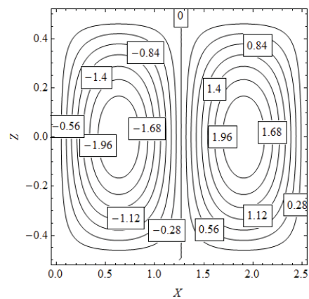
Fig. 6 Contour plot of Stream function for H = 10 , \sigma^2 = 10 , \Lambda = 1 , Pr = 4 , \phi = 0.88 , a_1 = 1.4 , A_{10} = 1 and \tau = 0.5
