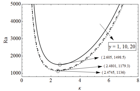
Fig. 4 Plot of Ra_l versus \kappa for different value of \gamma and for H = 10 , \sigma^2 = 10 , \Lambda = 1
