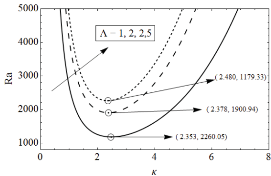
Fig. 3 Plot of Ra_l versus \kappa for different value of \Lambda and for H = 10 , \sigma^2 = 10 , \gamma = 20
