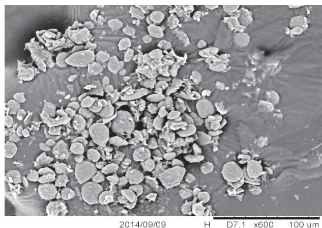
Fig. 6 SEM Image of Ginger Particles Produced by RESS-CO 2 Obtained at Extraction Temperature of 40°C and Extraction Pressure of 6000psi, 3.03 μm
