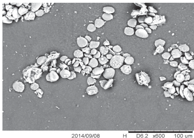
Fig. 5 SEM Image of Ginger Particles Produced by RESS-CO 2 Obtained at Extraction Temperature of 40°C and Extraction pressure of 5000psi, 2.22 μm
