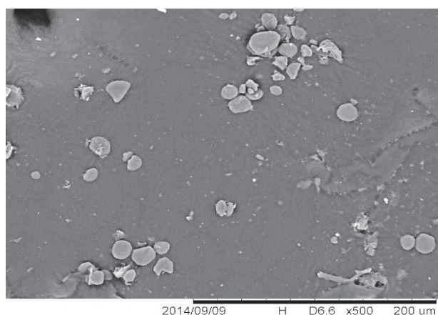
Fig. 3 SEM Image of Ginger Particles Produced by RESS-CO 2 Obtained at Extraction Temperature of 40°C and Extraction Pressure of 3000psi, 4.15 µm
