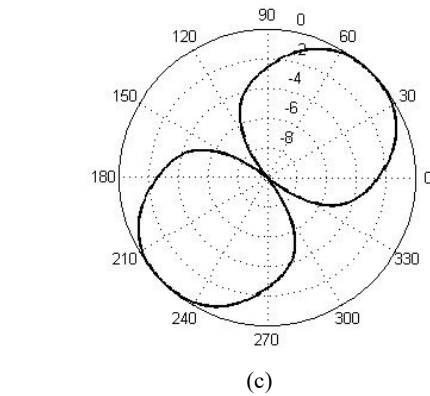
Fig. 7 (a) Configuration, (b) current distribution and (c) radiation pattern of case D
