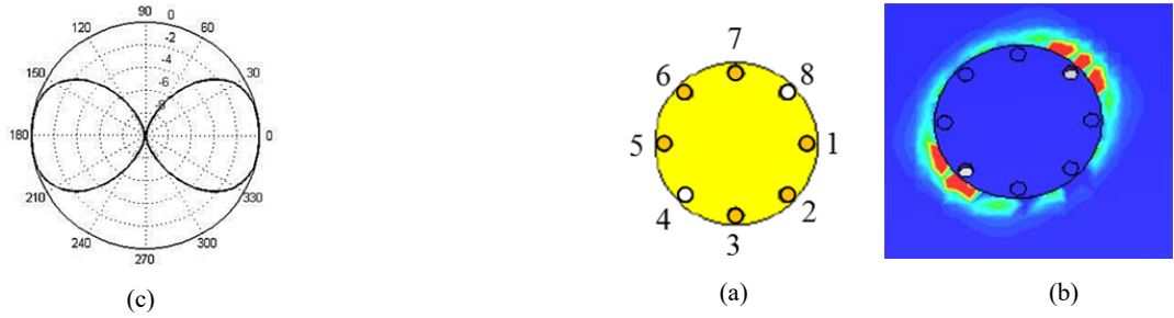
Fig. 4 (a) Configuration, (b) current distribution and (c) radiation pattern of case A
