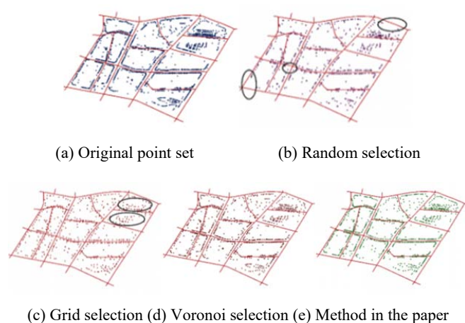
Fig. 4 Generalization Results
