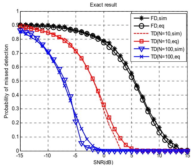
Fig. 6 P_m vs. SNR for exact analysis
