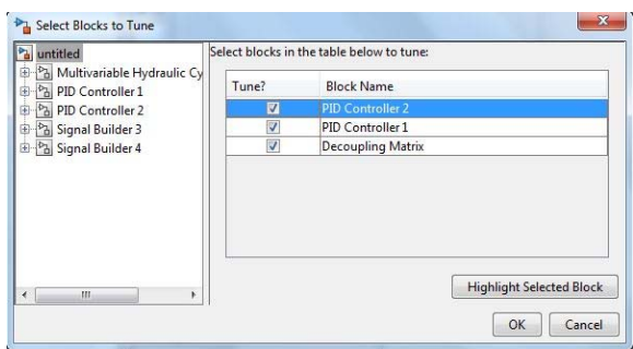
Fig. 7 SIMULINK PID controller tuner
