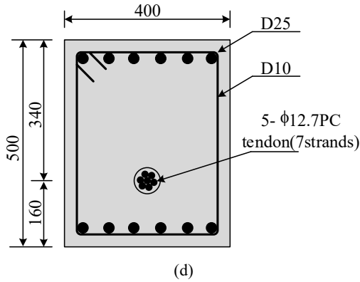
Fig. 2 Analyzed PSC beam (Unit : mm): (a) PSC420, PSC535a, and PSC 675a, (b) PSC535b, (c) PSC675b, and (d) beam section
