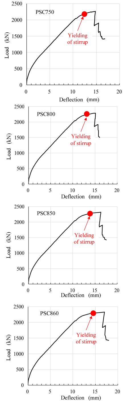
Fig. 4 Comparison of experimental and analytical load-deflection curves of PSC beams with various yield strength of stirrups
