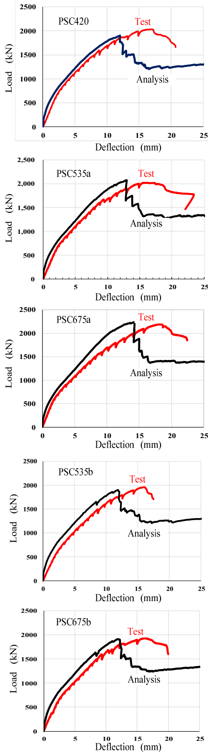
Fig. 3 Comparison of experimental and analytical load-deflection curves
