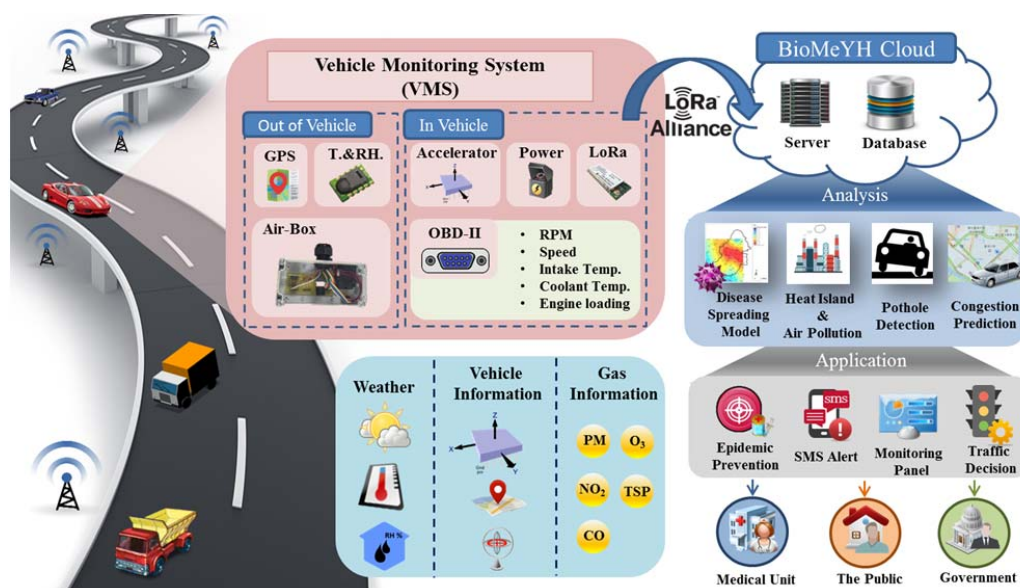
Fig. 1 The architecture of the VMS
