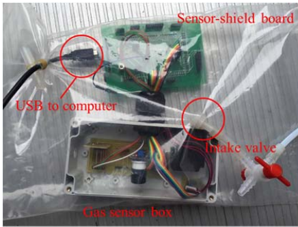
Fig. 12 The device used in the gas experiment
