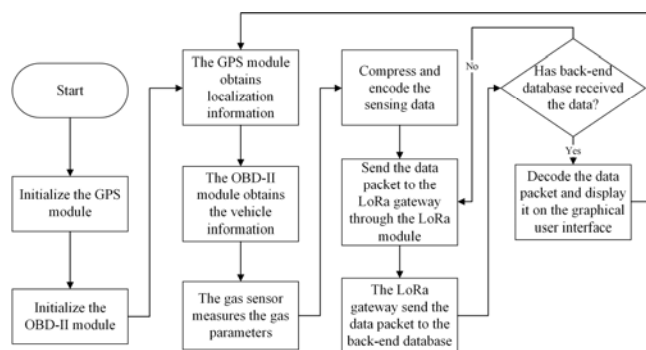
Fig. 11 The flowchart of the proposed monitoring system
