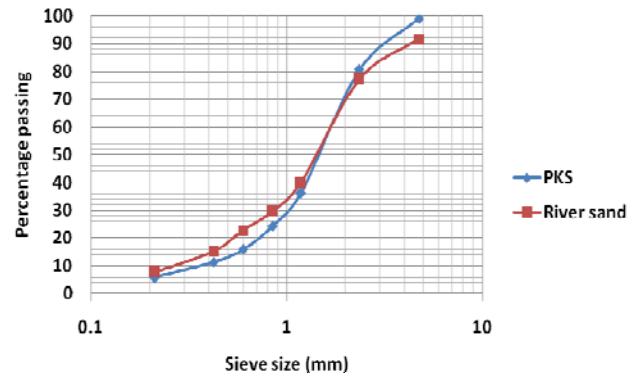
Fig. 3 Particle size distribution curves for PKS and River sand
