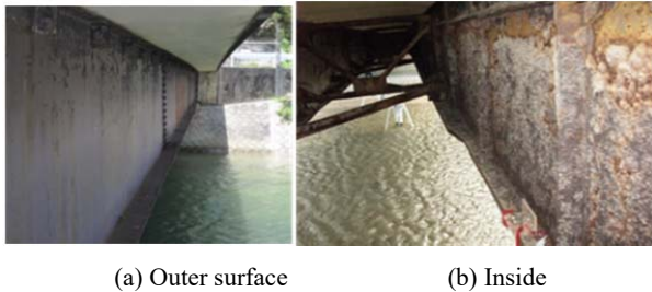
Fig. 3 Corrosion condition of bridge girders
