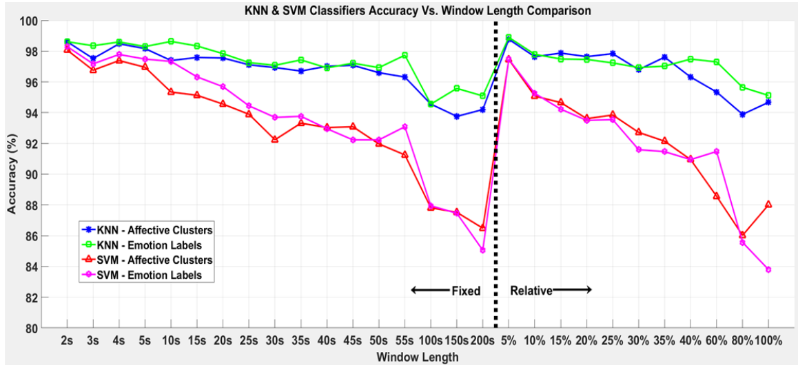
Fig. 3 KNN and SVM Classification Accuracy Comparison, vs. Window Lengths – According to Affective Clusters and Emotion Labels – The Horizontal Axes Presents 28 Window Lengths; 17 Fixed (Left Side of the Vertical Dashed Line) and 11 Relative (Right Side of the Vertical Dashed Line)
