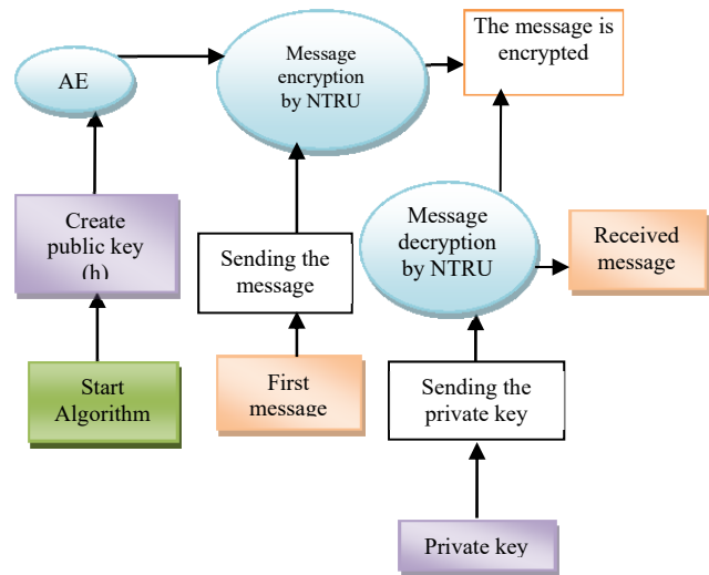
Fig. 2 HAN encryption algorithm steps sending public key
