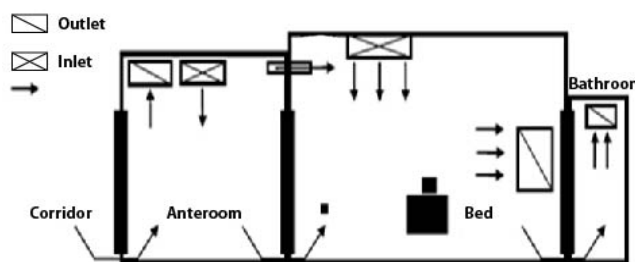
Fig. 1 Isolation room airflow
