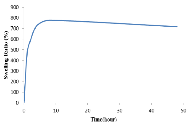
Fig. 4 Swelling ratio of sponges after two days
