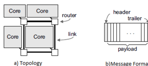
Fig. 1 NoC concepts [1]
