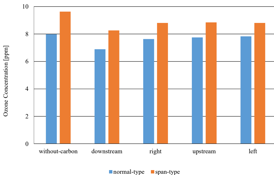
Fig. 16 Effect of carbon sheet on ozone concentration
