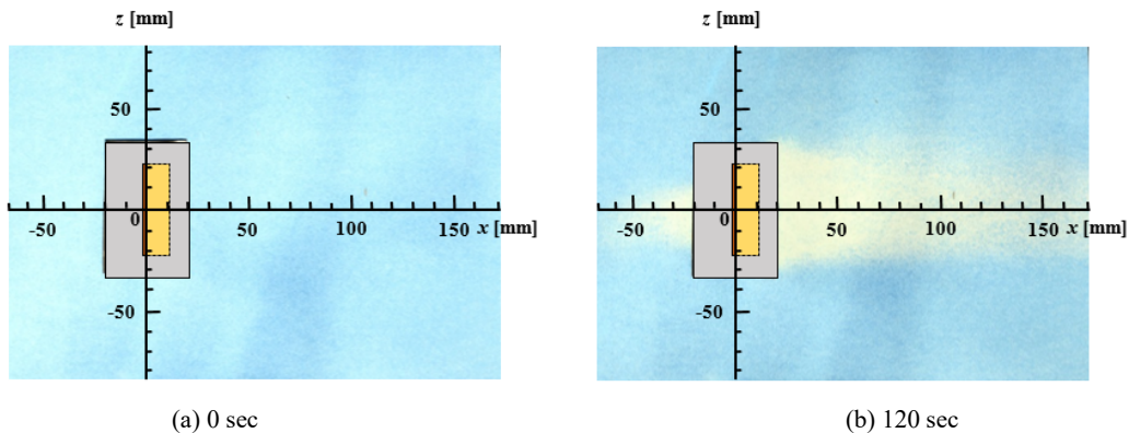
Fig. 12 Distribution of ozone in the x-z plane (span-type)
