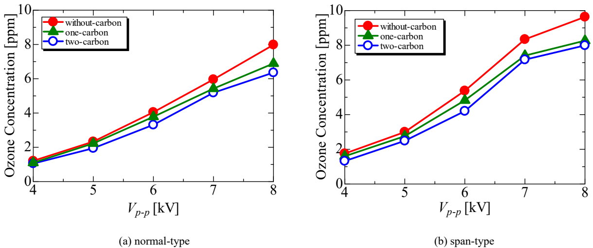
Fig. 20 Effect on number of carbon on ozone concentration
