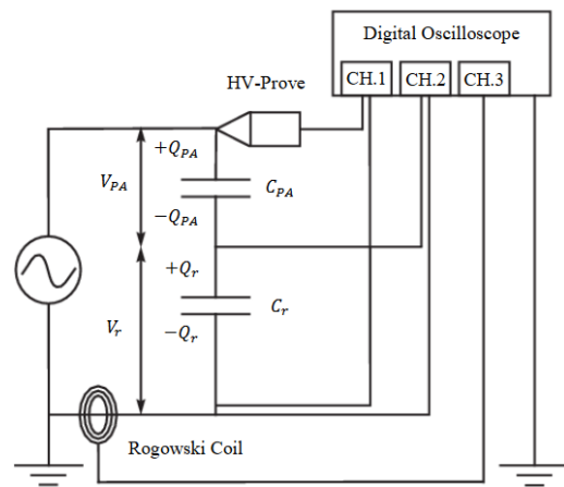
Fig. 5 Image of measuring power consumption
