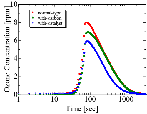
Fig. 17 Time variation of ozone concentration (normal-type, V_{p-p} = 8.0 kV, f_p = 5.0 kHz)
