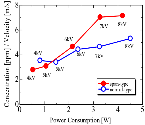
Fig. 10 Relation between concentration rate per velocity and power consumption
