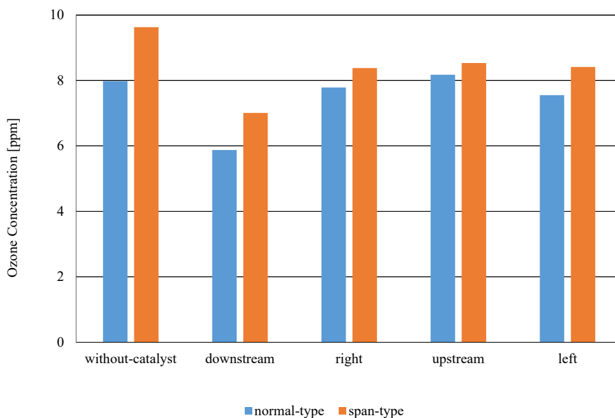
Fig. 15 Effect of honeycomb catalyst on ozone concentration
