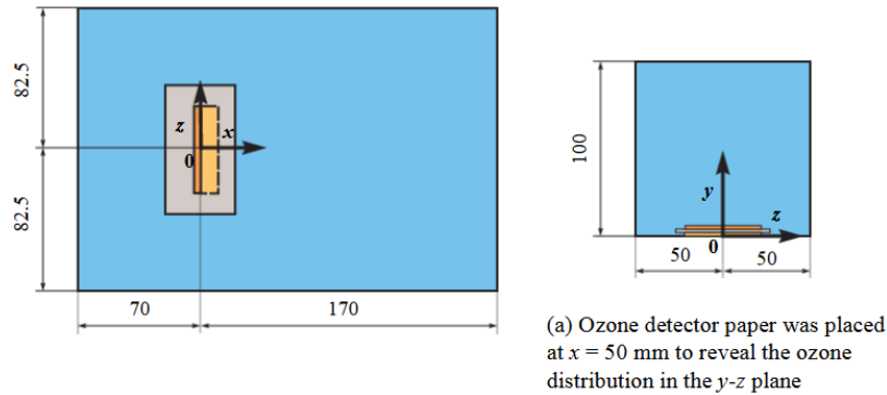
Fig. 6 Setting position of ozone detector paper
