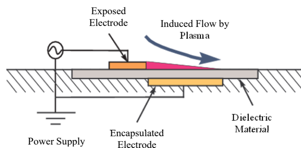
Fig. 1 Structure of DBD-PAs
