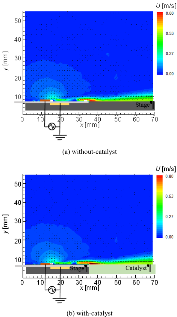
Fig. 21 Velocity profile (normal-type, V_{p-p} = 6.0 kV, f_p = 5.0 kHz)
