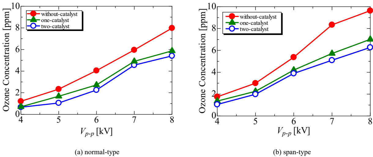
Fig. 19 Effect on number of catalyst on ozone concentration
