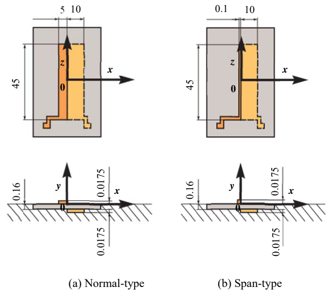
Fig. 2 DBD-PAs design
