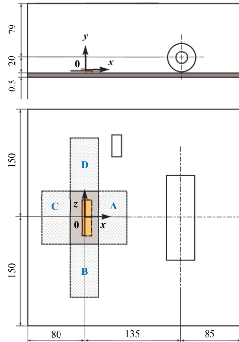
(b) To examine placement position, catalyst or carbon was placed as shown at a, b, c, d and ozone concentration was measured
