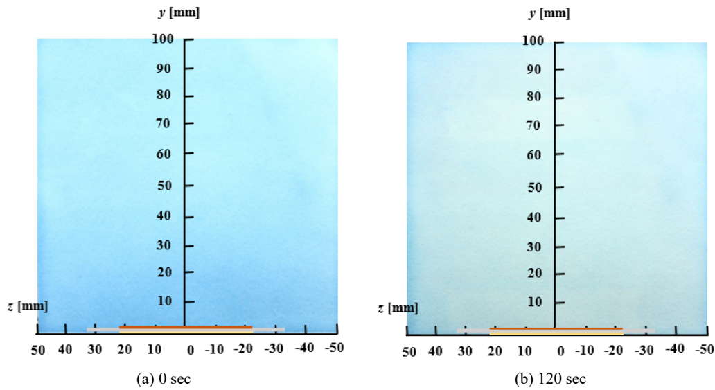
Fig. 13 Distribution of ozone in the y - z plane (normal-type, x = 50 mm)
