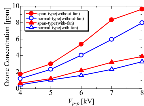
Fig. 9 Relation between ozone concentration and voltage
