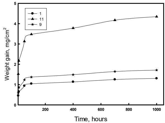
Fig. 7 The variation of mass gain ( \text{mg}/\text{cm}^2 ) with time (hours) of steels 1, 11 and 9 at 800 °C up to 1000 hour
