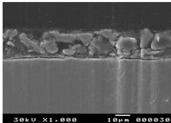
Fig. 14 SEM micrograph of steel (3)
