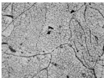
(c) Steel (2A) (Third group) 20X
