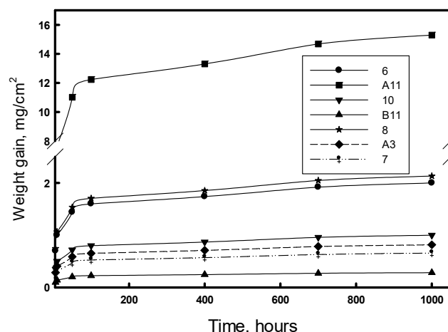
Fig. 9 The variation of mass gain (mg/cm 2 ) with time (hours) of steel grades of second group ( 6, A11, 10, B11, 8, A3 & 7) at 800 °C up to 1000 hour
