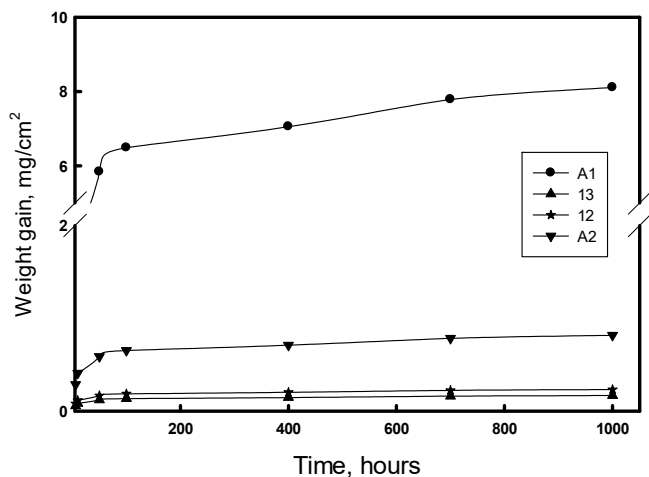
Fig. 11 The variation of mass gain (mg/cm 2 ) with time (hours) of steel grades of third group (A1, 13, 12, A2) at 800 °C up to 1000 hour
