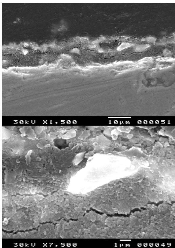
Fig. 12 SEM micrograph of steel (2)
