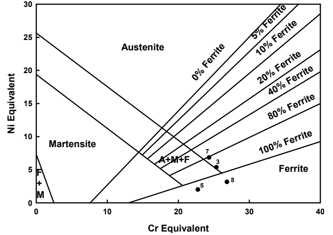
Fig. 6 Schaeffler diagram of fourth group, with (mass%), A= austenite, M martensite, F= ferrite of steels 7, 3, 8 & 5
