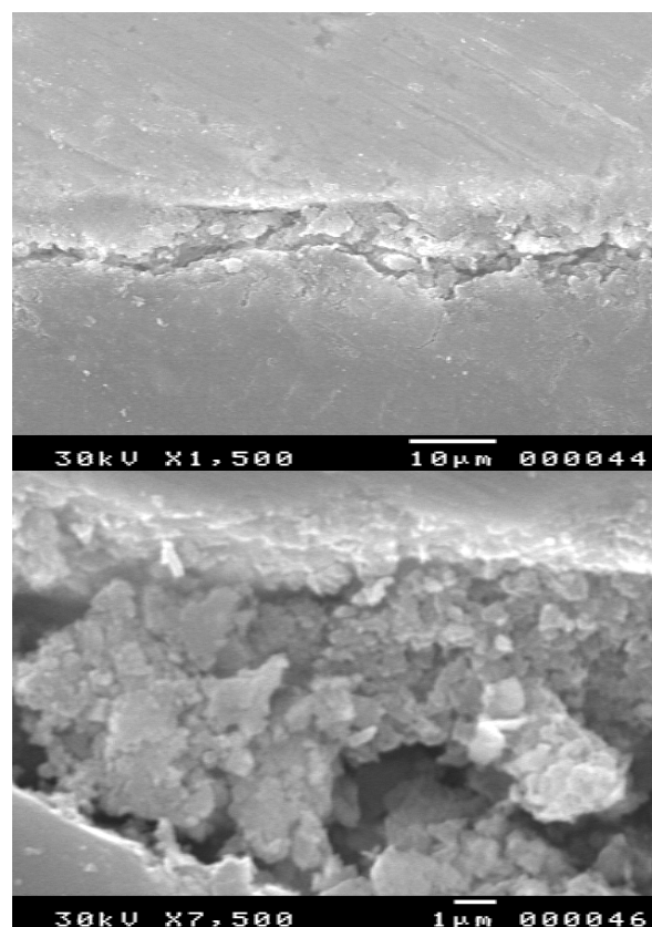
Fig. 10 SEM micrograph of steel (7)
