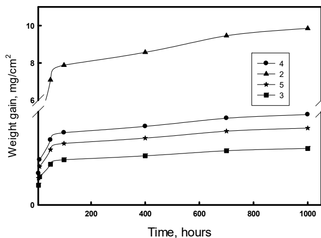
Fig. 13 The variation of mass gain (mg/cm 2 ) with time (hours) of steel grades of fourth group (4, 2, 5, 3) at 800 °C up to 1000 hour
