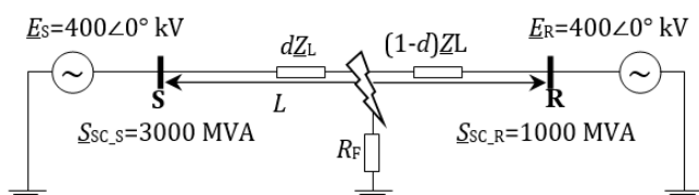
Fig. 6 One-line scheme of the test grid implemented in MATLAB
