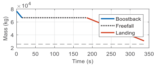
Fig. 13 Mass history for the 200-km downrange landing
