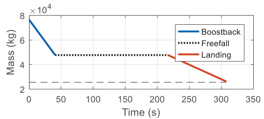
Fig. 17 Mass history for the return-to-launch-site landing
