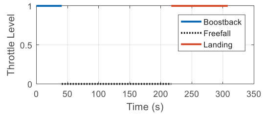
Fig. 16 Throttle control history for the return-to-launch-site landing
