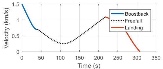
Fig. 18 Velocity history for the return-to-launch-site landing
