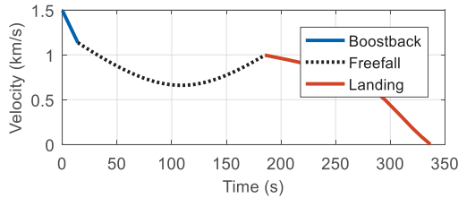
Fig. 14 Velocity history for the 200-km downrange landing
