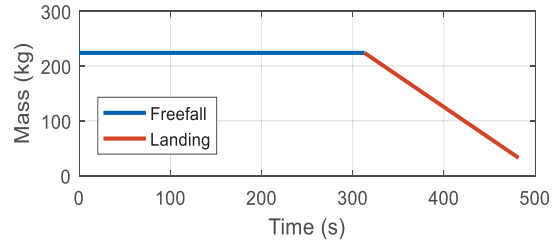
Fig. 6 Mass history from optimizing switching time and terminal time
