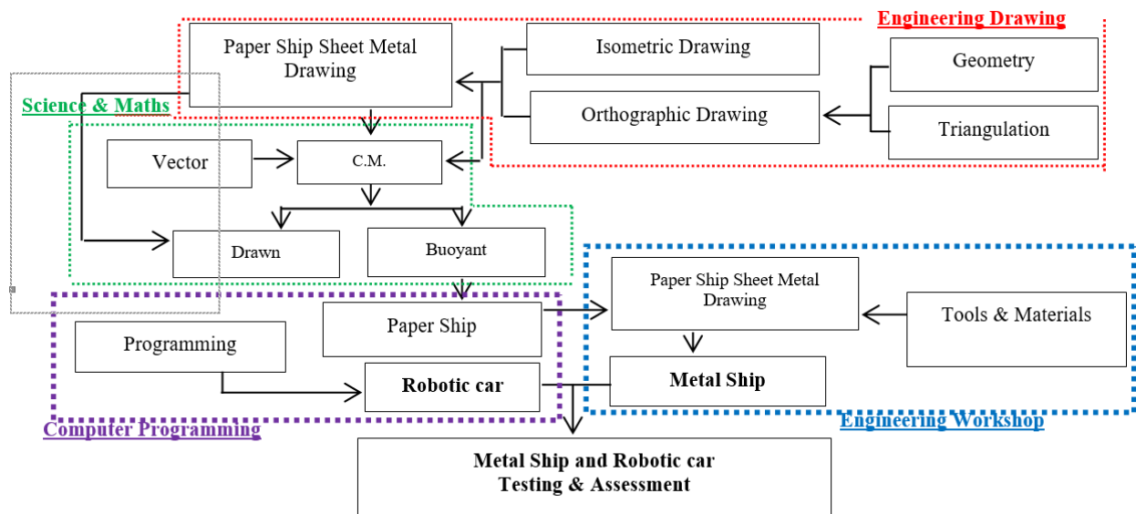
Fig. 1 Learning Process
