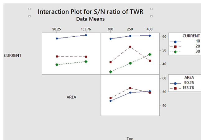
Fig. 9 Interaction Plot for S/N ratio of TWR
