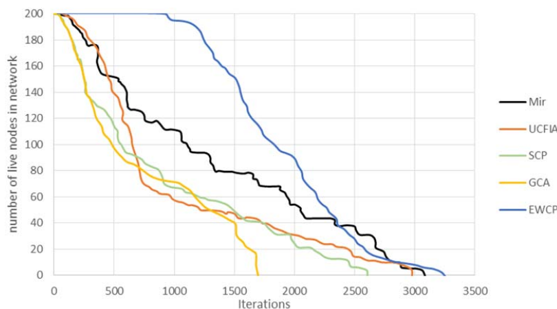
Fig. 4 Lifetime of network
