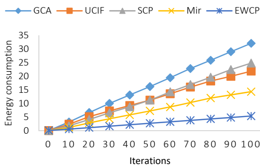
Fig. 3 Energy consumed in 100 iterations
