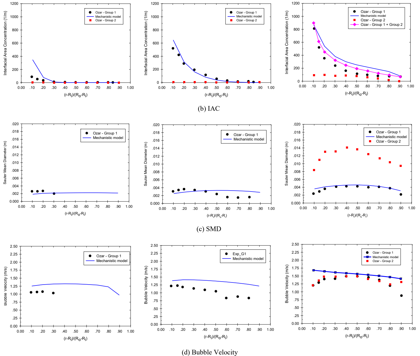
Fig. 5 Comparisons of local radial profiles of the considered parameters between the predictions the experiments for OZAR241 ( Q_{wall} = 241 \text{ kW/m}^2 , V_{inlet} = 1.02 \text{ m/s} , T_{sub} = 14.9 \text{ K} , P_{inlet} = 504 \text{ kPa} )
