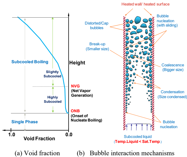
Fig. 1 Phenomenological descriptions of subcooled boiling flow
