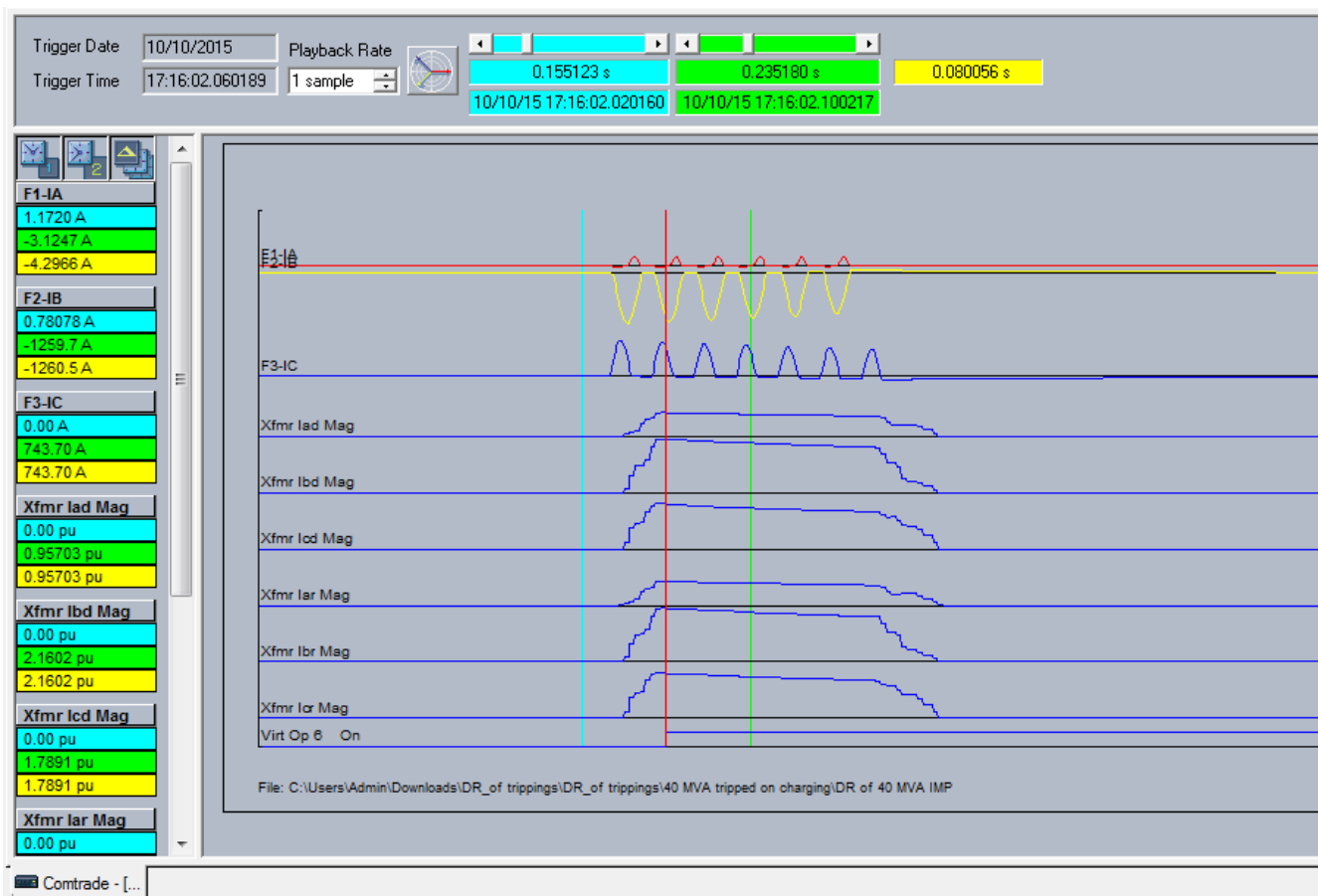
Fig. 1 Ratlam 40MVA Transformer – Tripped on healthy condition
