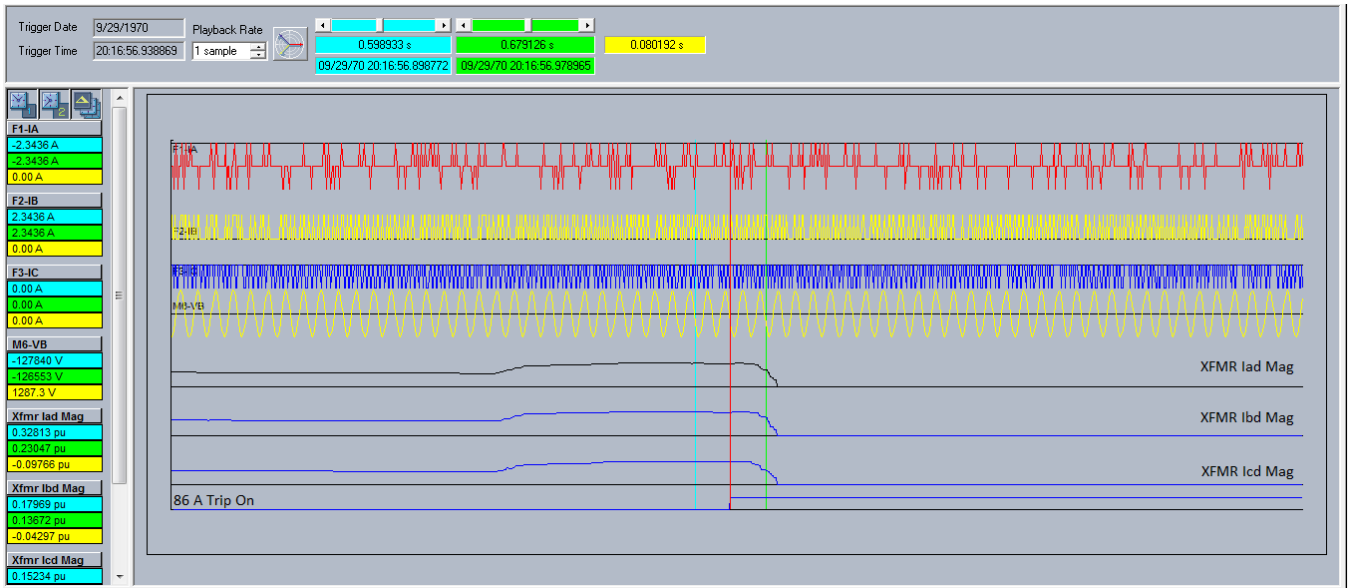
Fig. 3 Bina 315MVA Transformer – No trip for faulted condition
