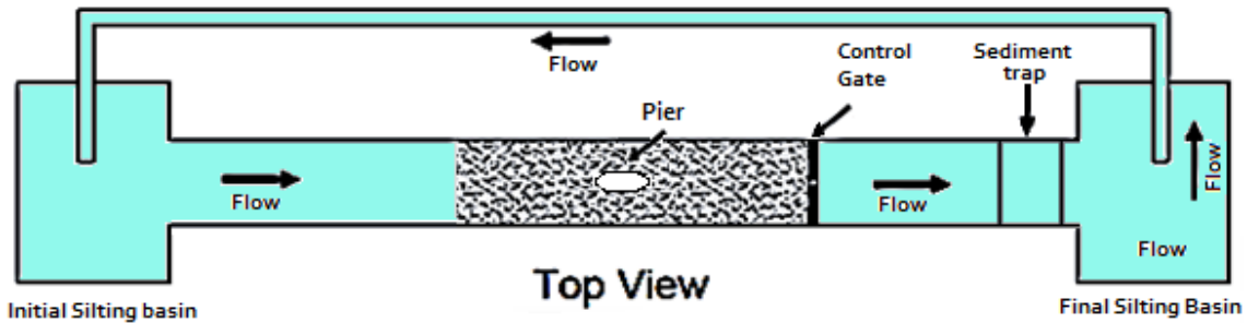
Fig. 4 (b) Top view of Experimental channel
