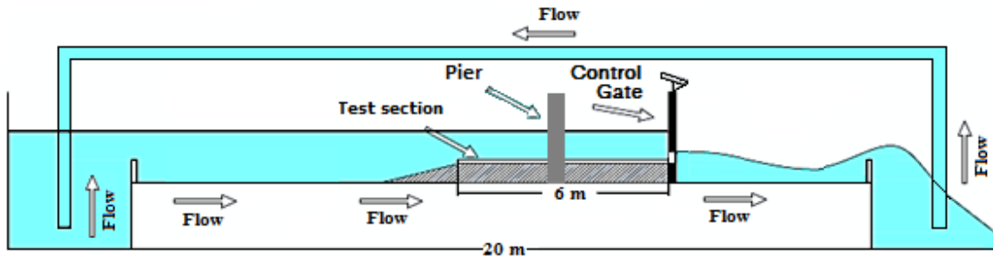
Fig. 4 (a) Cross section of Experimental channel
