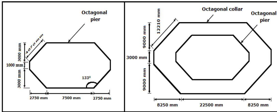
Fig. 2 Detail of pier & collar dimensions
