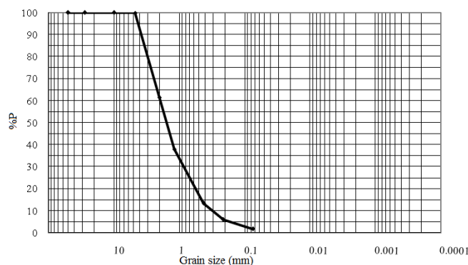
Fig. 2 Grain size distribution of the sand used in the tests
