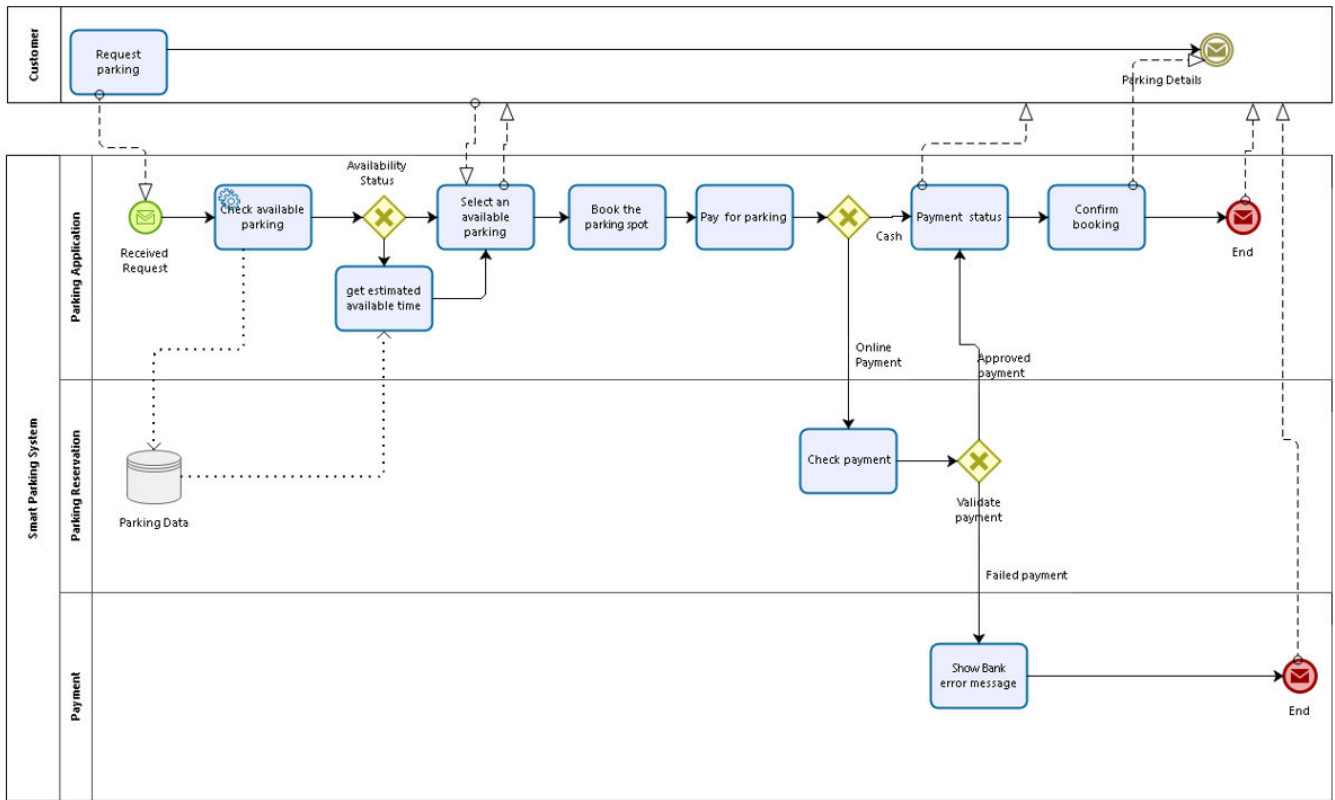
Fig. 1 Process model for smart car parking system
