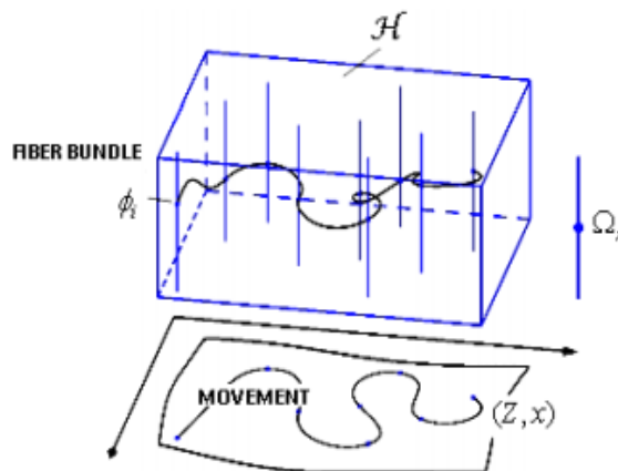
Fig. 1 Correspondences between states (L, \dot{x}) , of the Hamiltonian space \mathcal{H} , and points (Z, x) , of the loop space
