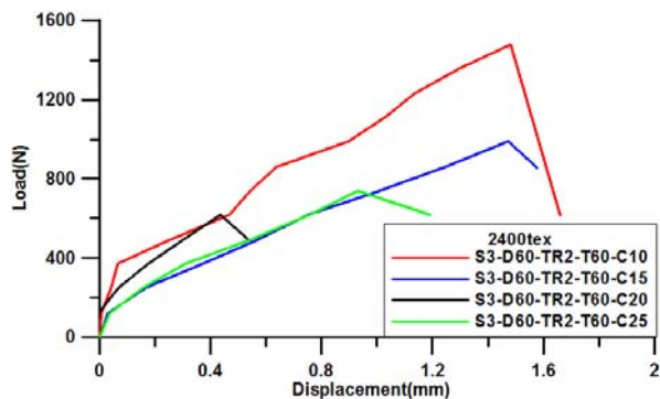
Fig. 3 Load according to lateral reinforcement spacing
