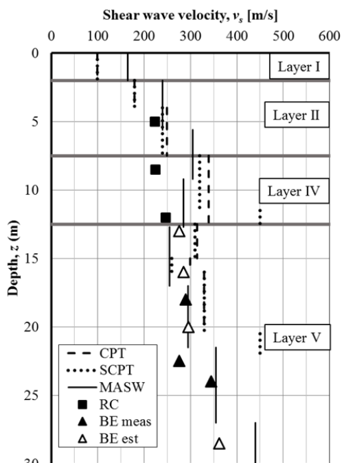
Fig. 8 Comparison of obtained shear wave velocity values
