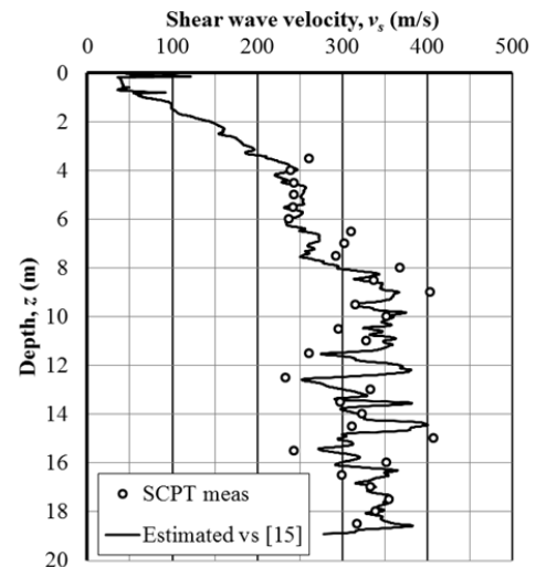
Fig. 4 Measured and estimated shear wave velocity profile
