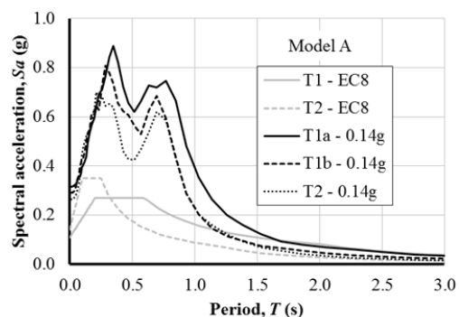
Fig. 10 Acceleration response spectra for different EQ motions
