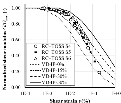
Fig. 7 Modulus degradation curves obtained with RC+TOSS tests
