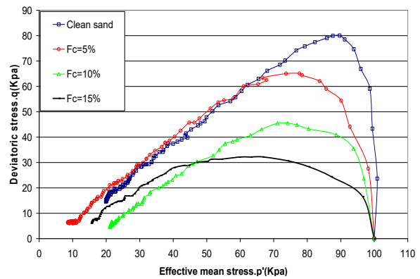
(b) Plot of stress paths
