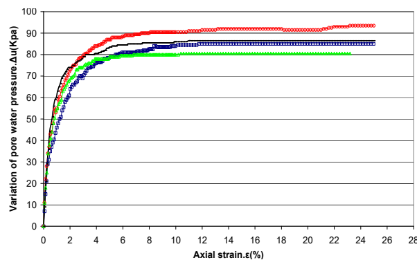
(c) Excess pore water against axial strain
