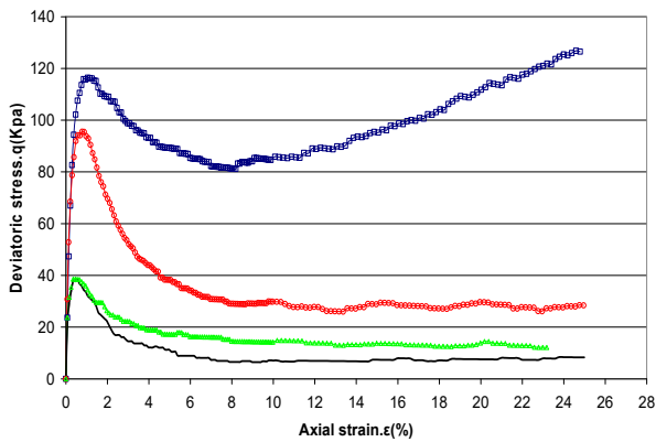
(a) Deviatoric stress against axial strain
