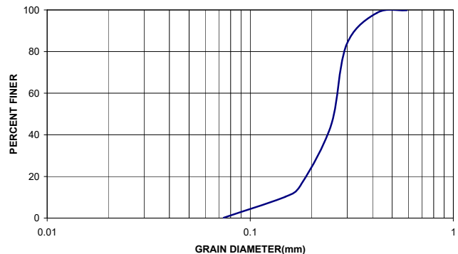
Fig. 1 Particle- size distribution of sand (161)
