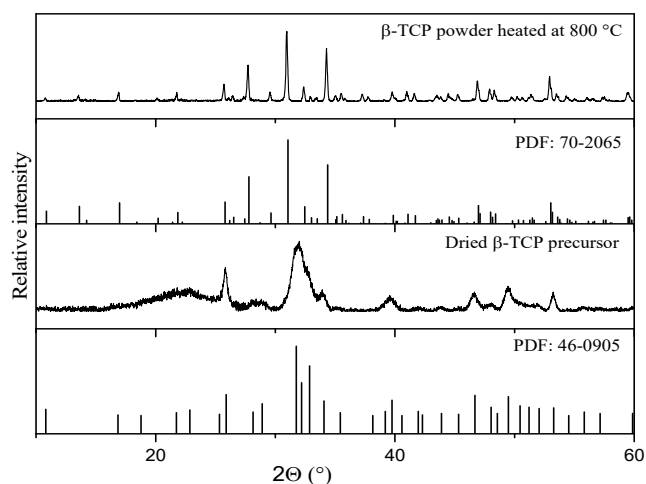
Fig. 3 XRD patterns of the dried Ca-P-O PVA precursor and final product obtained after annealing at 800 °C. Vertical lines represent standard XRD patterns of \beta -TCP (at top) and CHA (at bottom)
