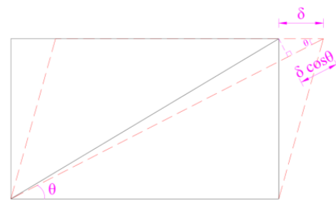
(b) Displaced model by earthquake force
