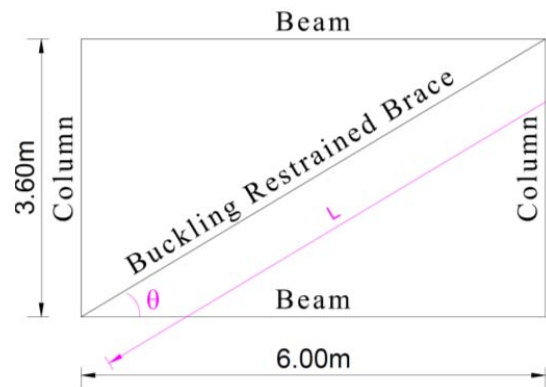
Fig. 6 Dimensions of the braced frame
