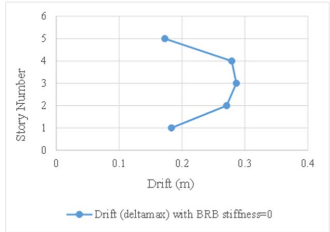
(a) Linear direct integration, time history analysis)
