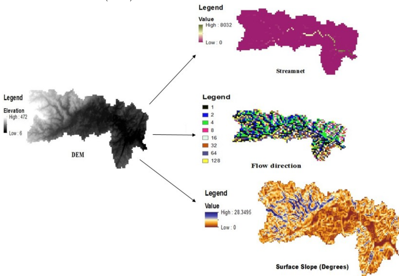
Fig. 4 Topographic data maps for PyTOPKAPI model input
