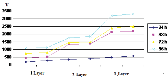
Fig. 7 The inception PD voltages for paper
