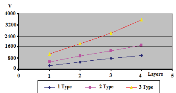
Fig. 8 The inception PD the 3 types of paper impregnated with drying
